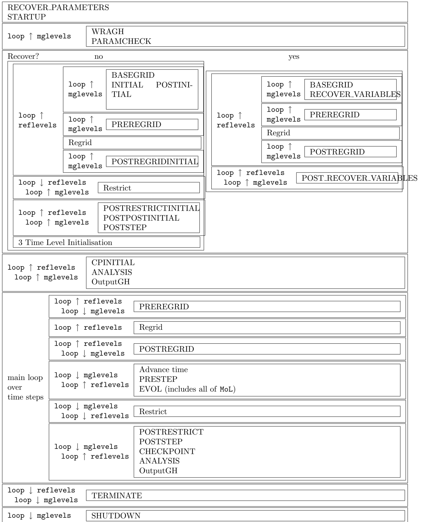
Figure 5: This figure gives a detailed description of how Carpet uses the Berger-Oliger algorithm to sequence through the schedule bins and grids (see figure 4 for a summary of the algorithm). ↑ loops iterate upwards on mglevel or reflevel, i.e. (for reflevel) from coarse grids to fine grids. ↓ loops iterate downwards on mglevel or reflevel, i.e. (for reflevel) from fine grids to coarse grids. At present mglevels aren't used, i.e. the mglevels loops have only a single iteration. Erik: ES: The postre-grid bin loops now over all time levels. The initial bin can also do this if init_all_timelevels is selected. Erik: ES: Some of these loops may have change recently. Check.
